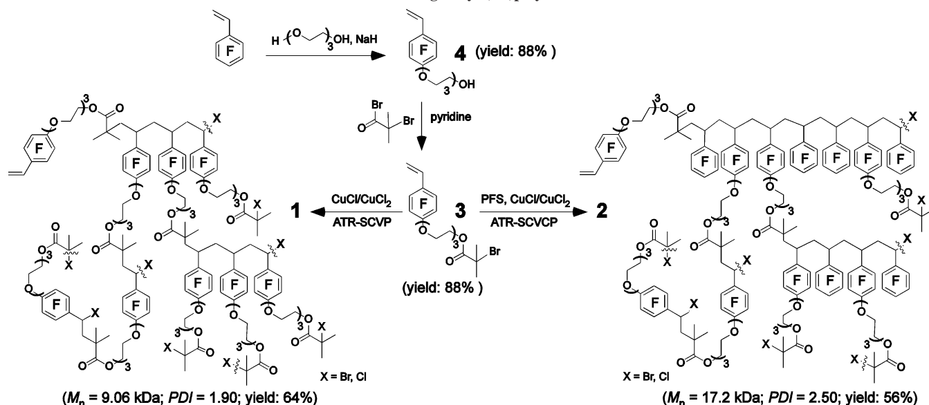
Scheme 1. Syntheses of Hyperbranched Fluorohomopolymer 1 and Fluorocopolymer 2 by Atom Transfer Radical Vinyl Self-Condensing Vinyl (Co)polymerization
