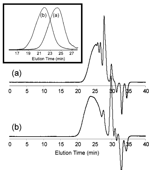
Figure 1. SEC traces for (a) homopolymerization of 3 at t = 10 h and (b) copolymerization of 3 and PFS at t = 8 h, with SEC traces of the final purified polymers 1 and 2 ( t = 24 h) included as insets.
