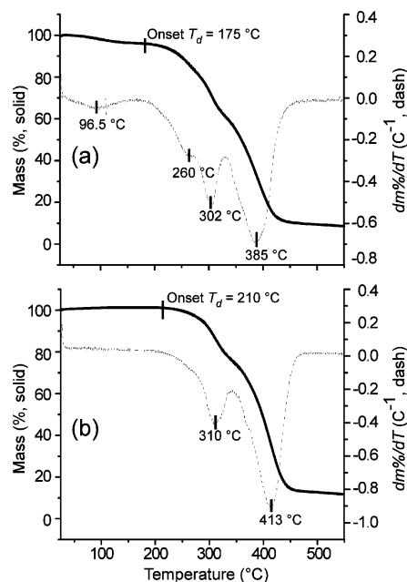
Figure 5. Thermolytic profiles for (a) hyperbranched fluorohomopolymer 1 and (b) hyperbranched fluorocopolymer 2 . Mass % is illustrated with solid lines and the first-derivative plots are shown as dashed lines.
